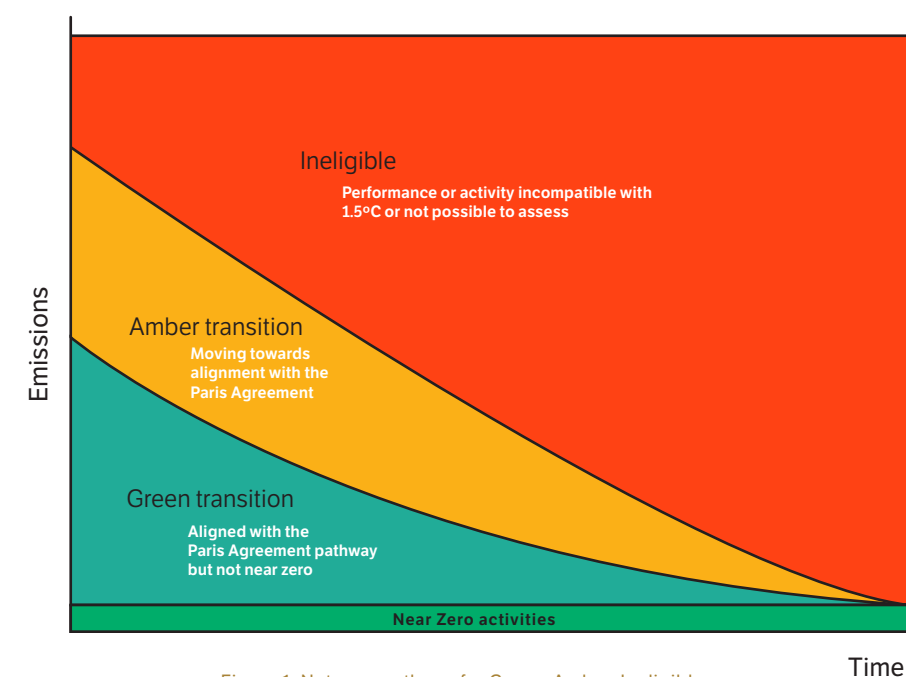
Figure 1: Net-zero pathway for Green, Amber, Ineligible
