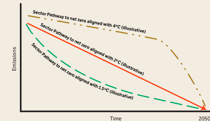
Figure 2: Illustrative 2050 pathways aligned with a range of temperatures
