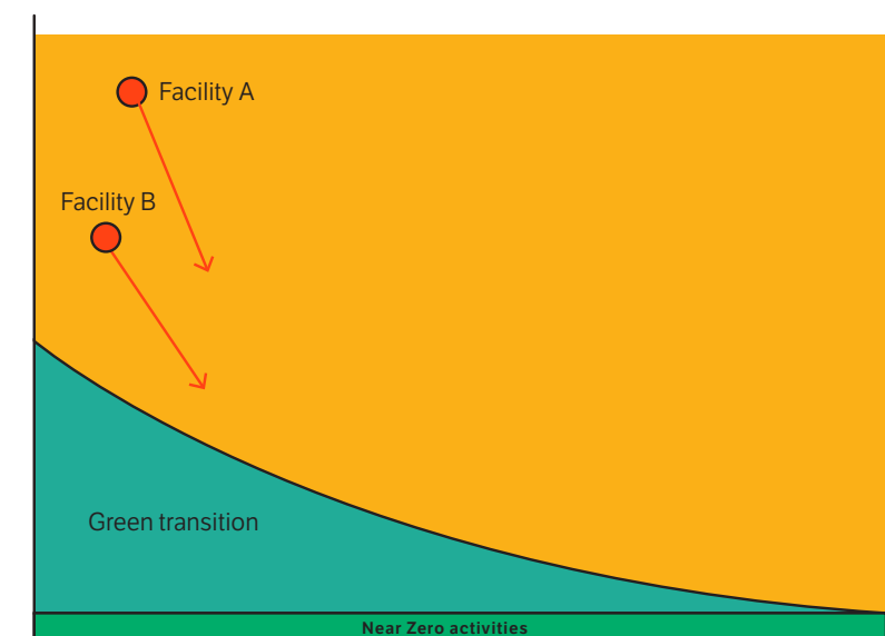
Figure 8: Amber category for industry sectors
