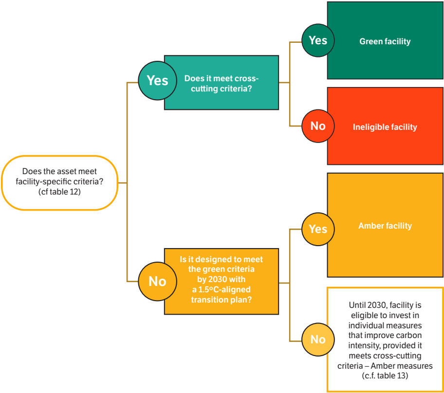
Figure 11: Eligible categories for iron and steel production – a high level overview
